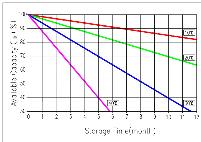
■ Curve of Self-discharge at Different Temperature
