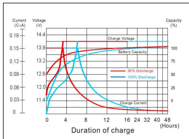
■ Constant Voltage Charge Characteristics
